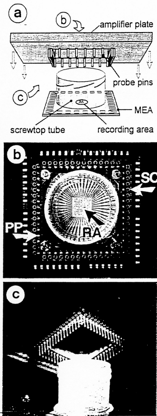
Fig. 4. MEA hardware. (A) Schematic representation of MEA chamber and amplifier plate. The plate is equipped with 60 probe pins at the bottom, which contact the outer MEA strip conductor pads when the plate is lowered onto the MEA. The screwtop tube is inserted into the central opening of the amplifier plate. Labels indicate views depicted in (B) and (C). (B) Top view of the MEA chamber attached to the amplifier plate. The set of 60 small holes (SC, stimulus connector) are designed to house pins to connect the stimulus isolation unit. Beside each stimulus connector the top of the corresponding probe pin (PP) is visible. The recording area (RA) is in the very center of the MEA. (C) Lateral perspective before lowering the amplifier plate with probe pins onto the MEA with attached screwtop tube. MEA dimensions are 5 × 5 cm.
