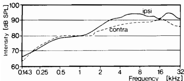
Fig. 1. The frequency response of the closed sound system. The graph is representative for all experiments and shows the sound pressure level (re 2.10^{-5} N/m 2 ) as a function of frequency at 0dB attenuation. Relative sound levels in the Figures represent dB attenuation relative to this level
